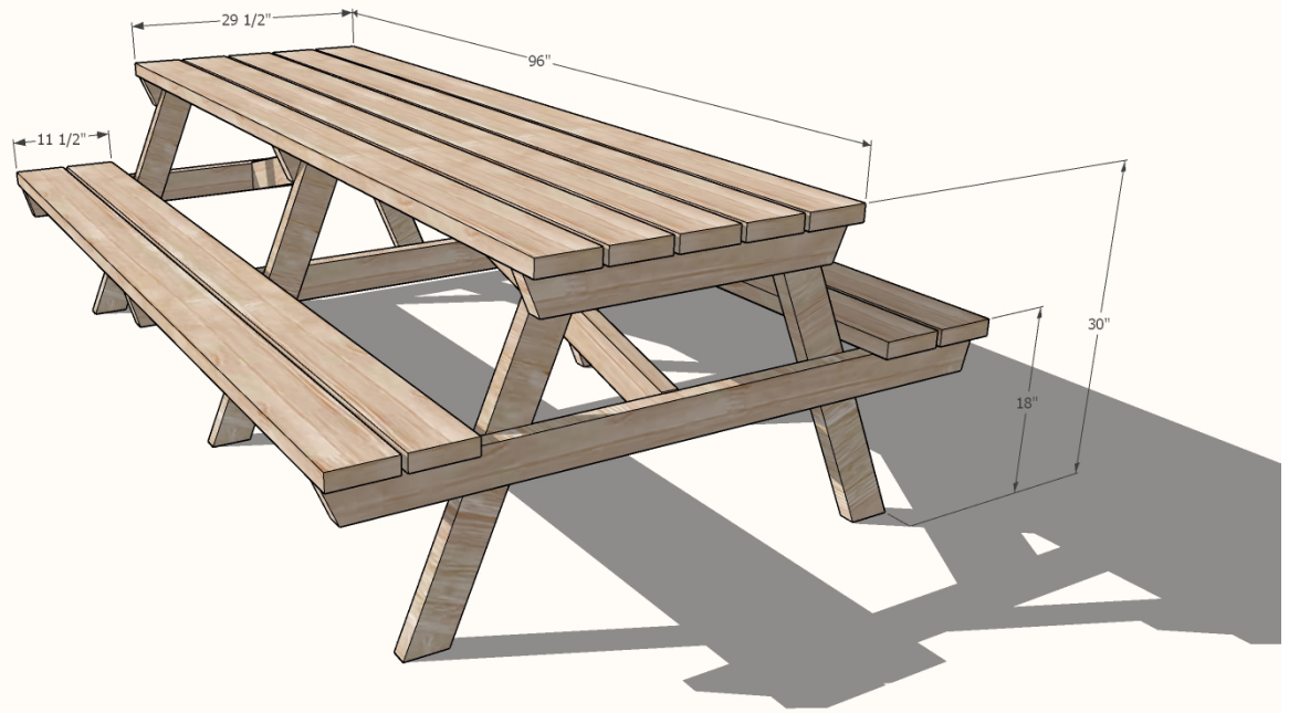
Picnic table plans dimensions
